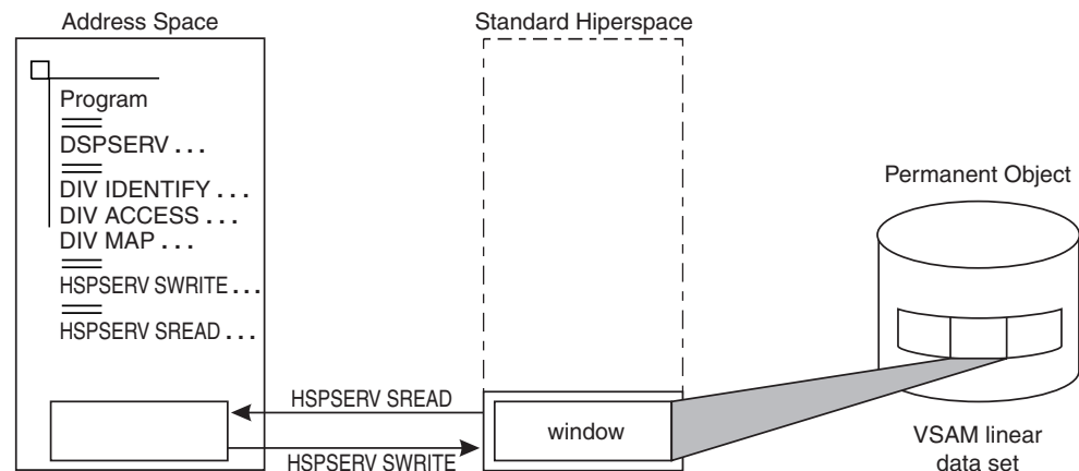
Figure 7-13. Example of Mapping a Data-in-Virtual Object to a Hiperspace
