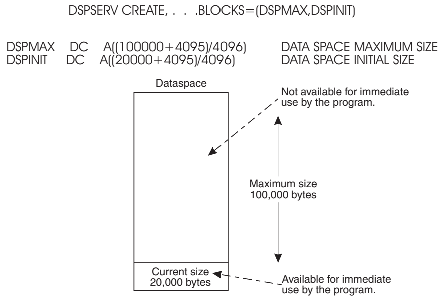
Figure 6-2. Example of Specifying the Size of a Data Space
