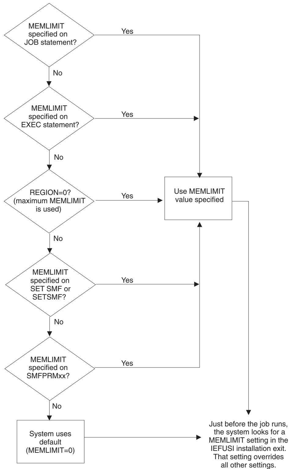
Figure 4-2. How the System Chooses which MEMLIMIT Applies
